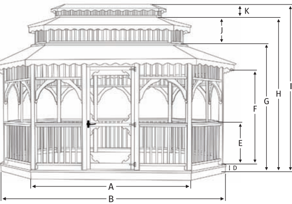
Oval Double Roof Gazebo
