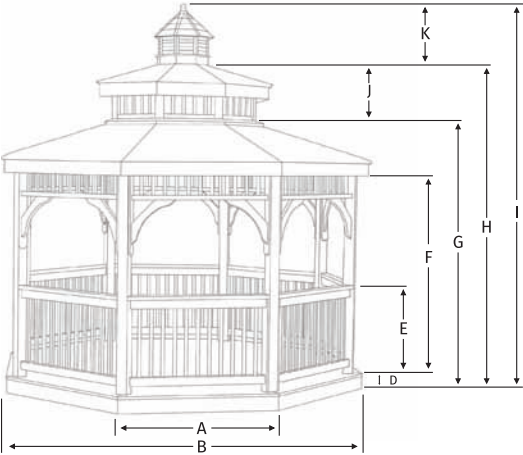
Octagon Double Roof Gazebo
